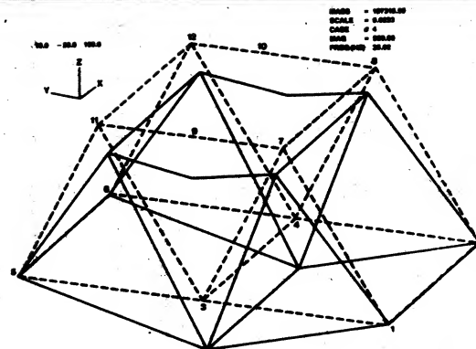
▲ CLASSICAL TRUSSEL BRIDGE. Visual recognition of dynamic mode shapes or deformations is easy with STRUSAP Graphics.
